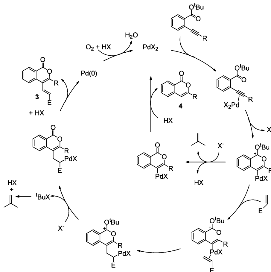
Scheme 4. Proposed Mechanism for the Formation of Isocoumarins
