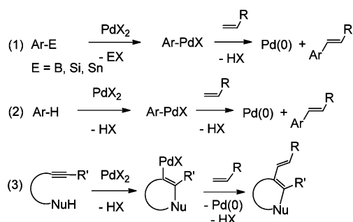
Scheme 1. Organopalladium Species in Oxidative Olefination
