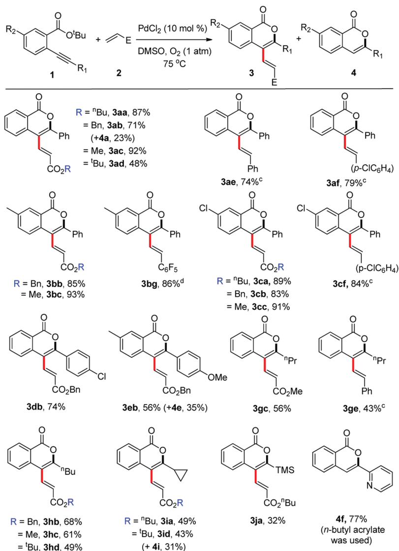
Scheme 3. Cyclization–Oxidative Olefination of tert -Butyl ortho -Alkynylbenzoates a,b
